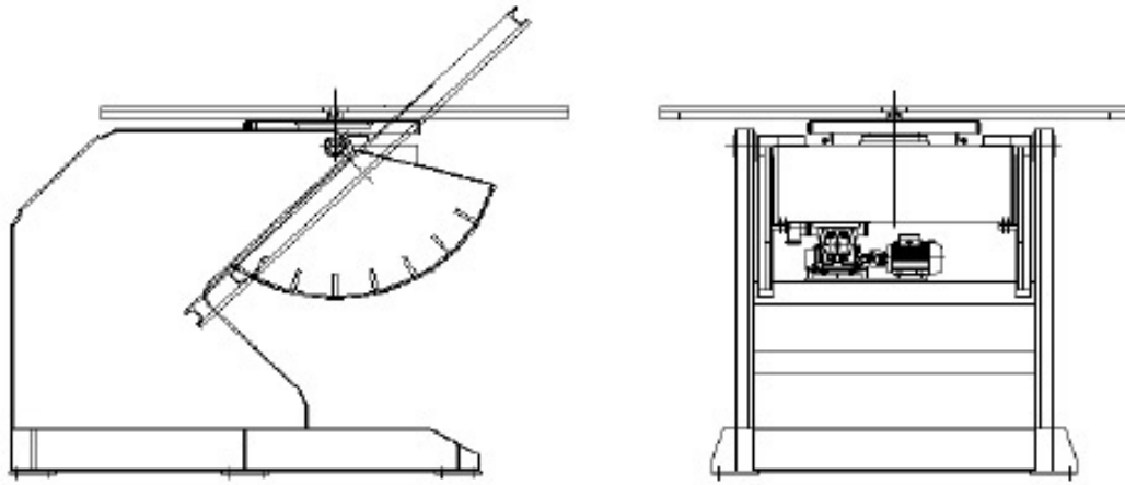
WELDING POSITIONER SPECIFICATION SHEET
